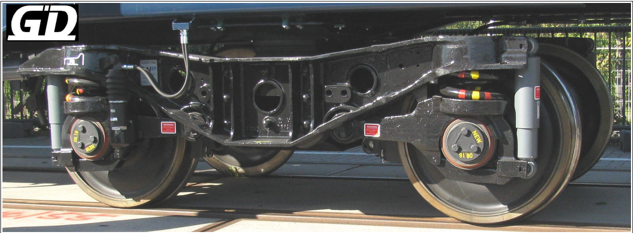
Güterwagen-Drehgestell Axiom LN 25 UK, unter 81 70 GB -VTGUK 5500 292-4 Ealnos (60 m 3 JNA), Astra Rail Freight Car Bogie Axiom LN 25, used with 81 70 GB -VTGUK 5500 292-4 Ealnos (60 m 3 JNA), Astra Rail
